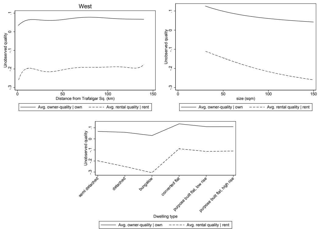
Figure 7: Unobserved quality
